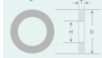
Drawing Notation
